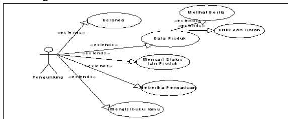
Gambar 1 Use Case
